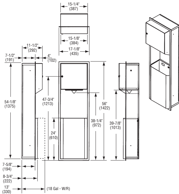
Recessed Mounted
