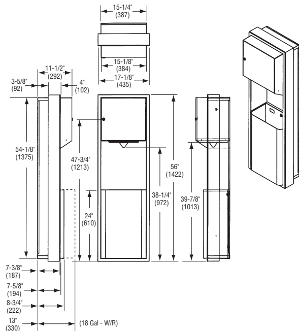
Semi-Recessed Mounted
